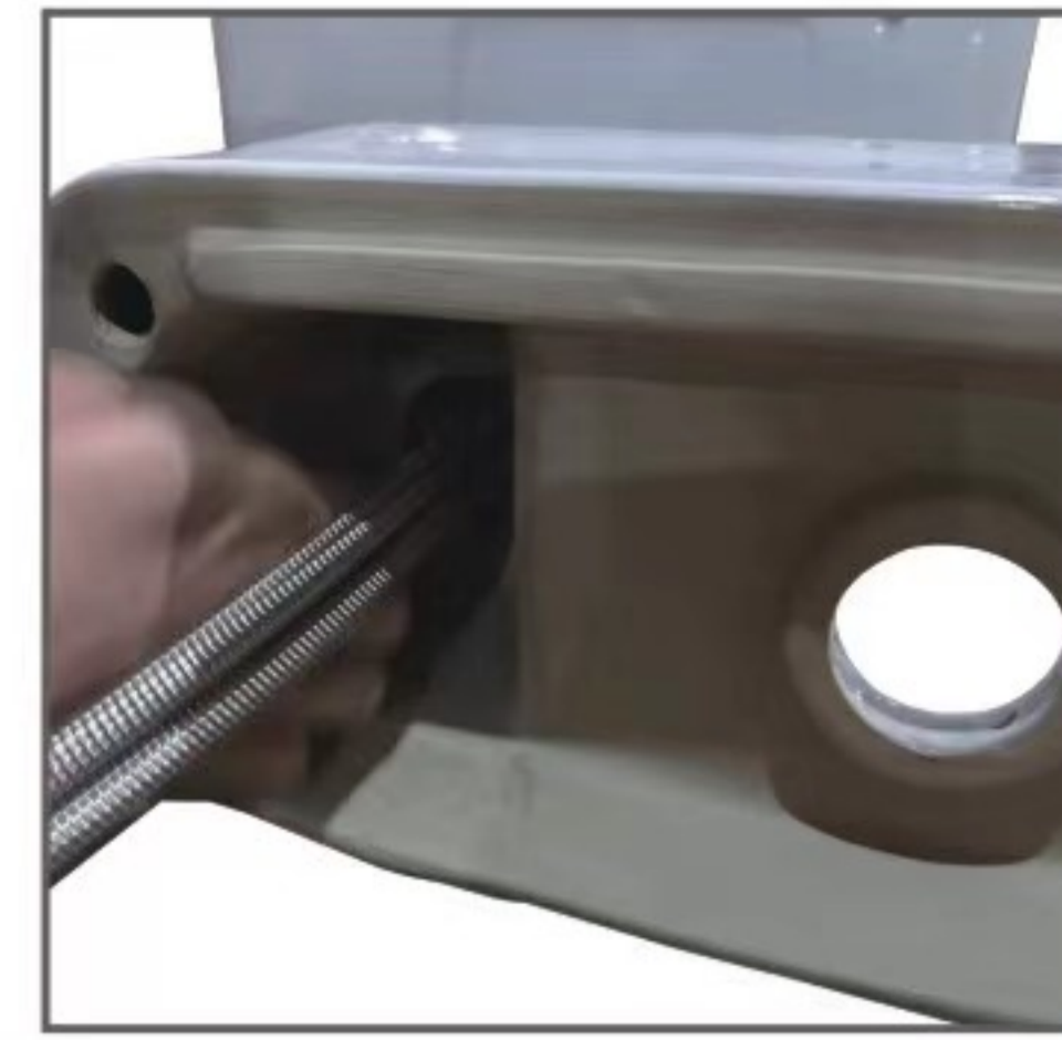
2-5: Install the faucet on the basin and connect the inlet pipe.
